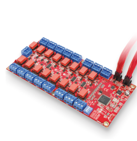
996540PCB&K Integriti UniBus 16 Floor Lift Interface device PCB & Accessories (Includes 270mm UniBus patch cable)
