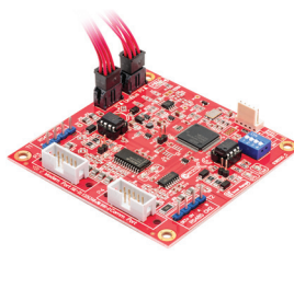
996520PCB&K Integriti UniBus 2 Port RS-232/RS-485 UART PCB & Accessories (Includes 270mm UniBus patch cable)
